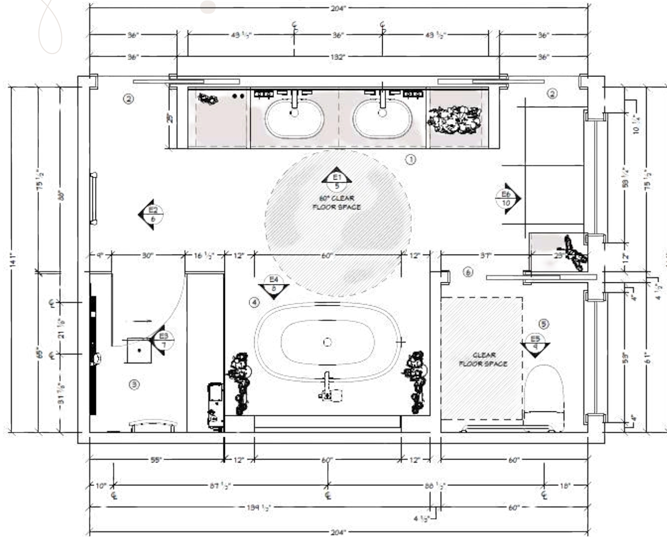
FLOOR PLAN SCALE 3/8" = 1'
