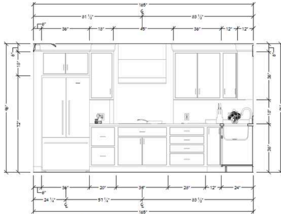
○ ELEVATION 1 SCALE 3/8" = 1'
