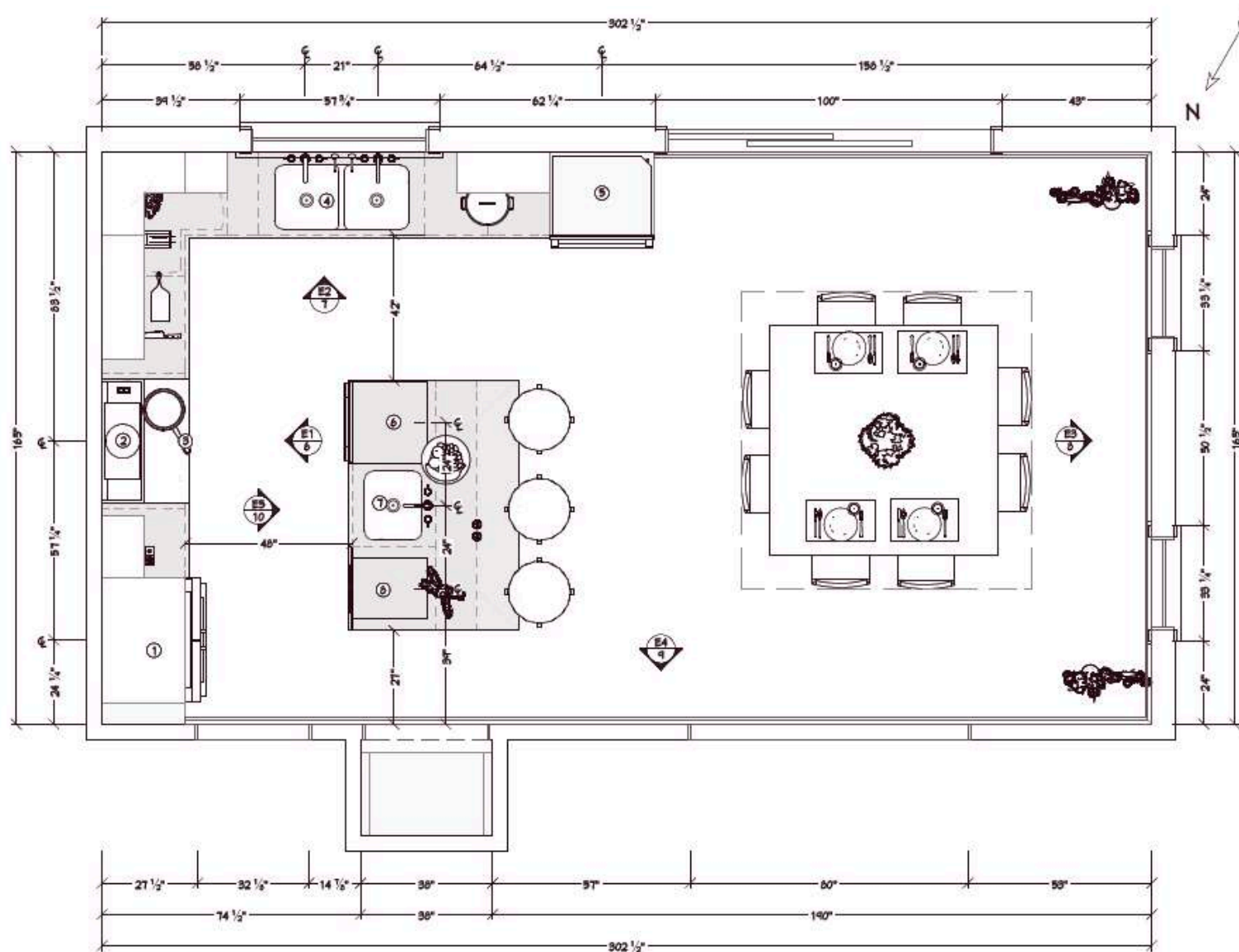
FLOOR PLAN SCALE 3/8" = 1'
